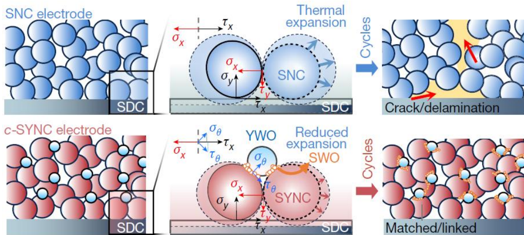
Thermal-expansion behavior engineering for SOCs
