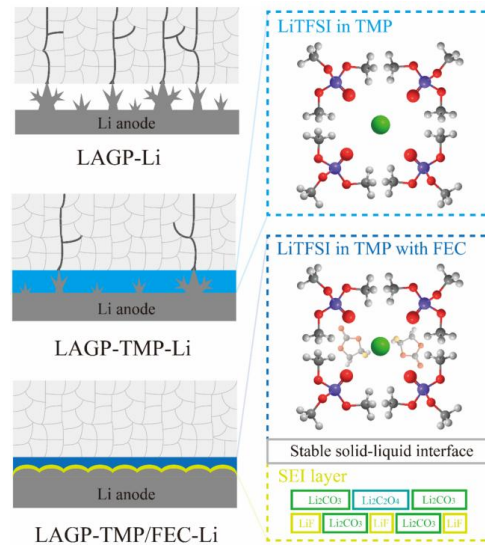
Interface engineering for SSBs
