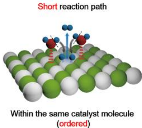
Reaction path engineering for HER
